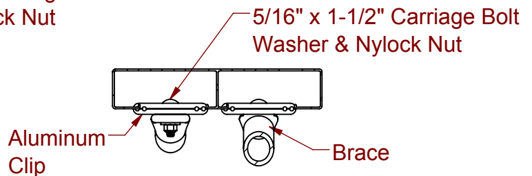
M2 ALUMINUM CLIP BRACE INSTALL
