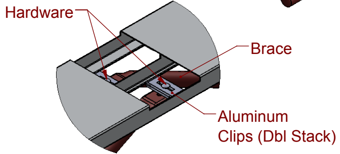
M2 ALUMINUM CLIP BRACE INSTALL
