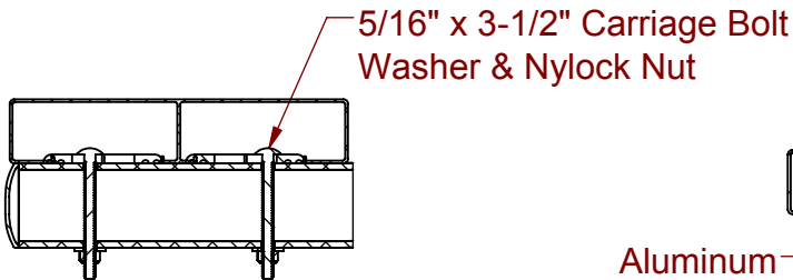
M2 ALUMINUM CLIP FRAME INSTALL
