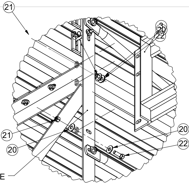
DETAIL-T ENLARGED
