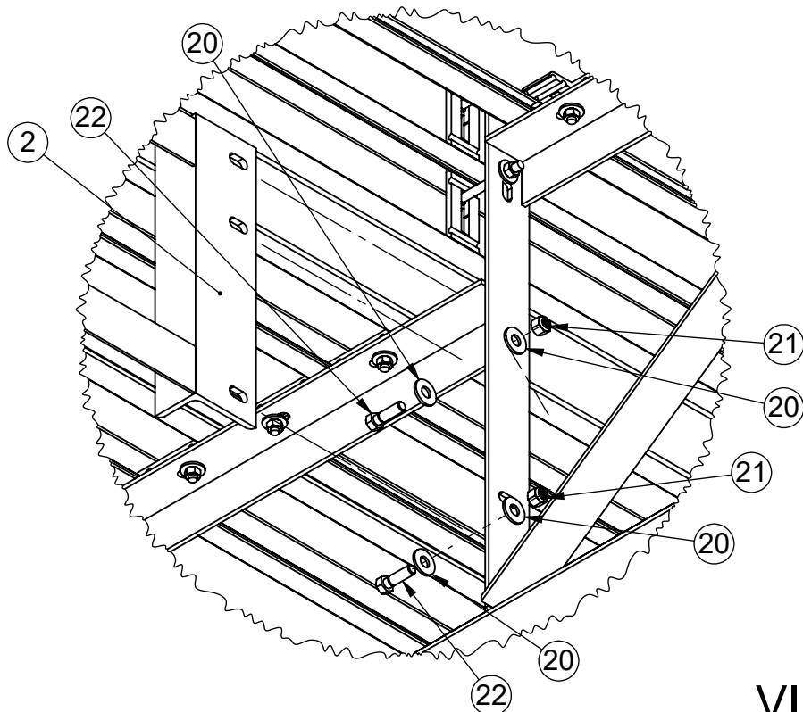
DETAIL-S ENLARGED
