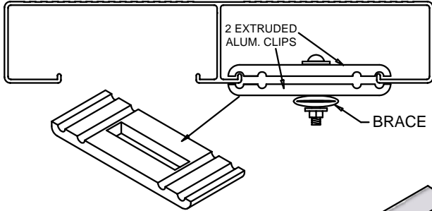
BRACE ATTACHMENT TO SEAT DETAIL - B
