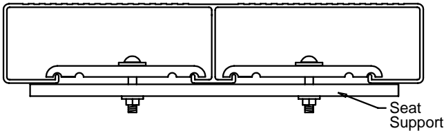
BRACE ATTACHMENT TO SEAT DETAIL - B
