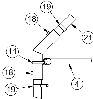
DETAIL E
