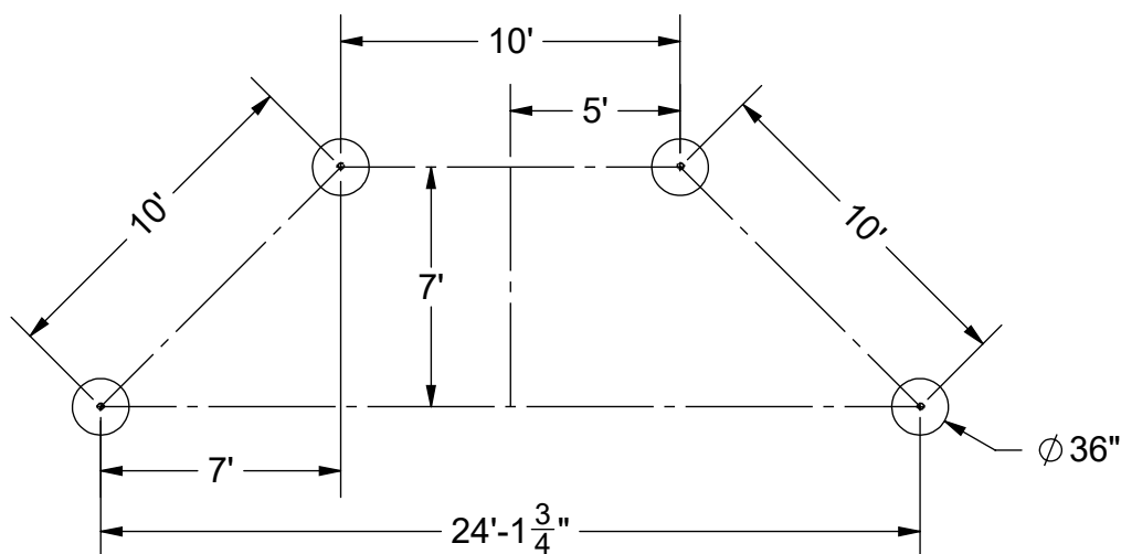
FOOTING DIMENSIONS
