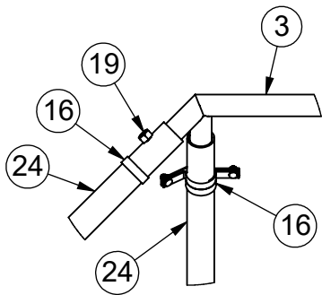
DETAIL D
