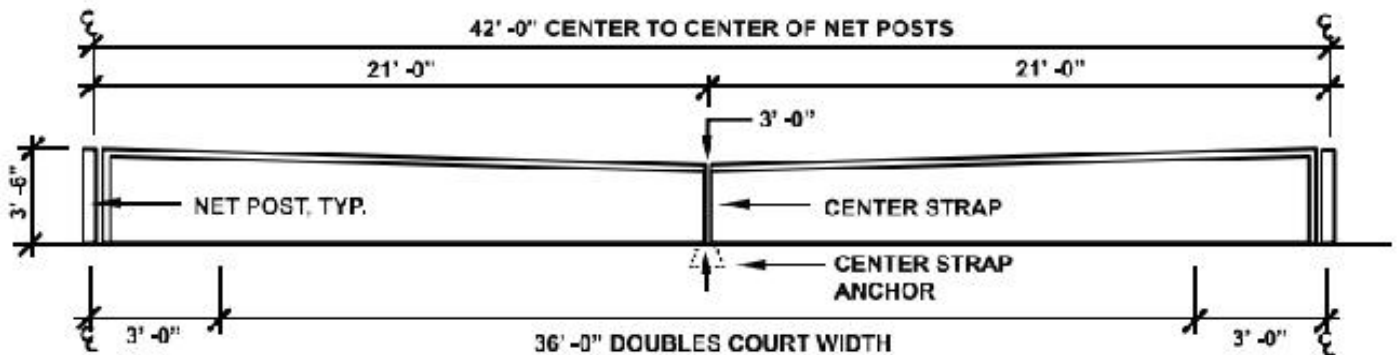
Typical Tennis Net Elevations
