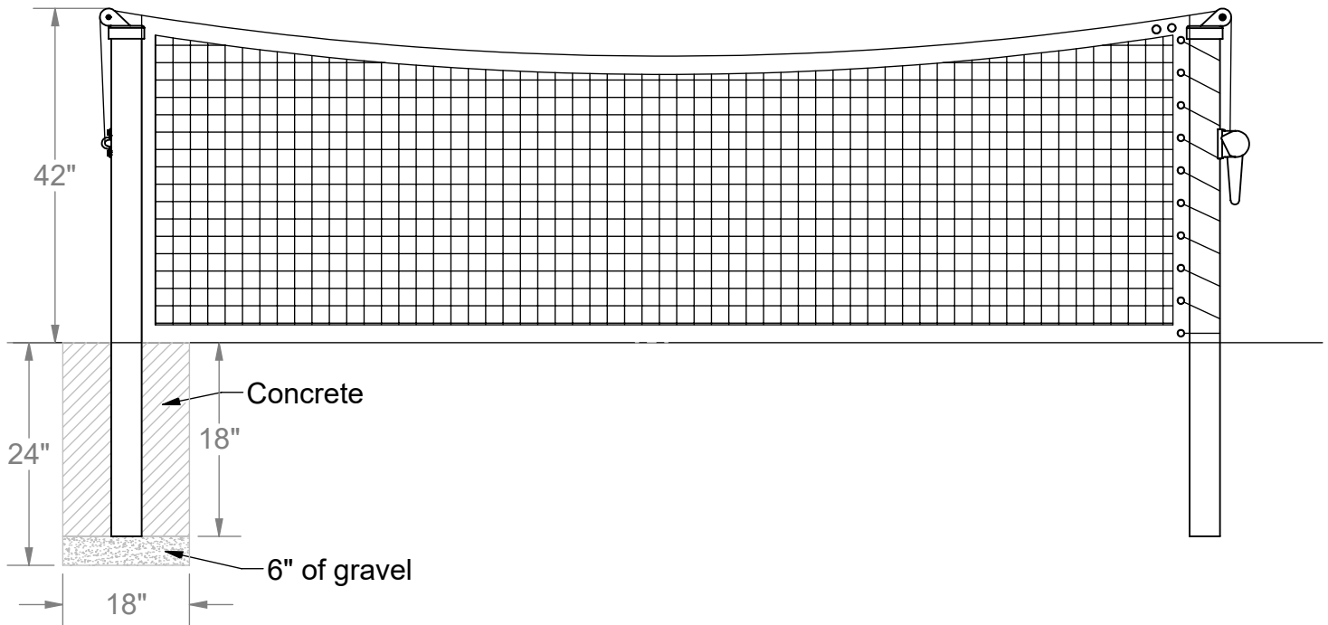
Typical Tennis Net Elevations
